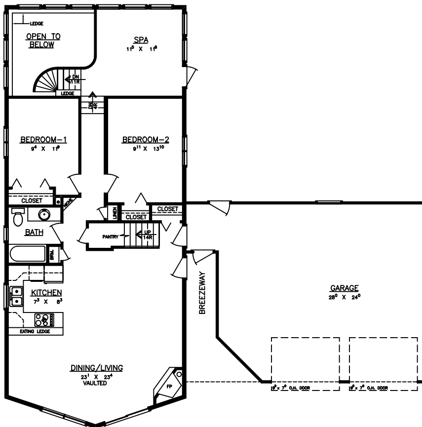
MAIN FLOOR AREA = 1302 S.F.
